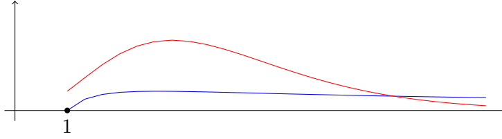
FIGURE 2. Graphs of x^3/e^x and \log(x)/x for x \in [1, 10] .
