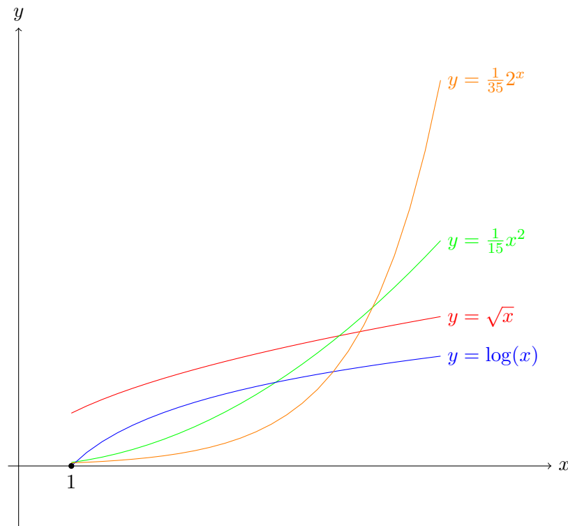
FIGURE 1. Graphs of several functions for x \in [1, 10] .
