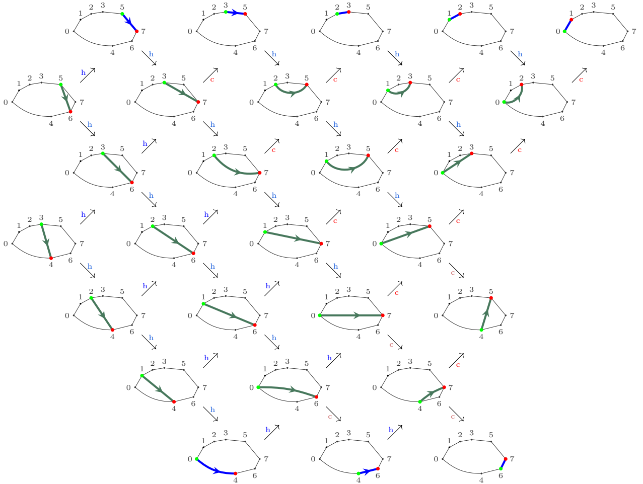
FIGURE 5. Auslander–Reiten quiver \Gamma_{\text{rep} Q} of \text{rep } Q for the quiver Q in Figure 1.
