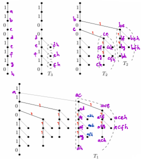
FIGURE 4. Bottom-up construction of \mathcal{T}_{L_2}(11001110) .
