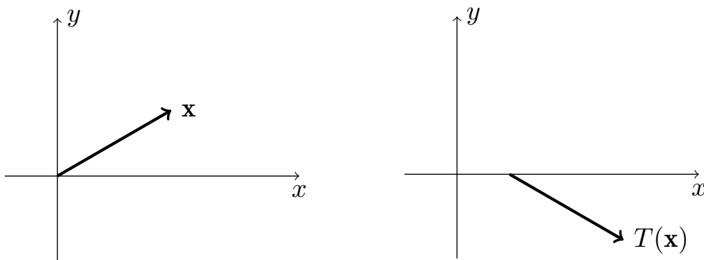
Figure 12.12 Glide reflections
