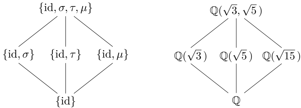
Figure 23.22 G(\mathbb{Q}(\sqrt{3}, \sqrt{5})/\mathbb{Q})
