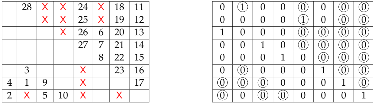
Figure 3: Left: The projection \Pi_c of Example 5.1. Right: permutation matrix for b_4 of Example 5.5.
